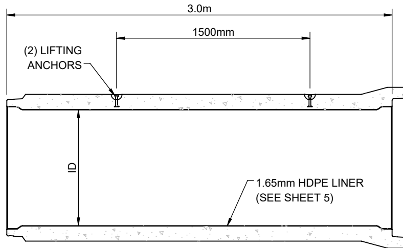
SECTION VIEW
