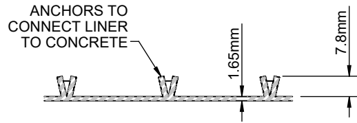
HDPE LINER DETAIL WITH ANCHORS
