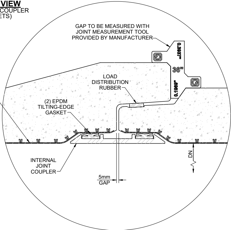
JOINT DETAIL
