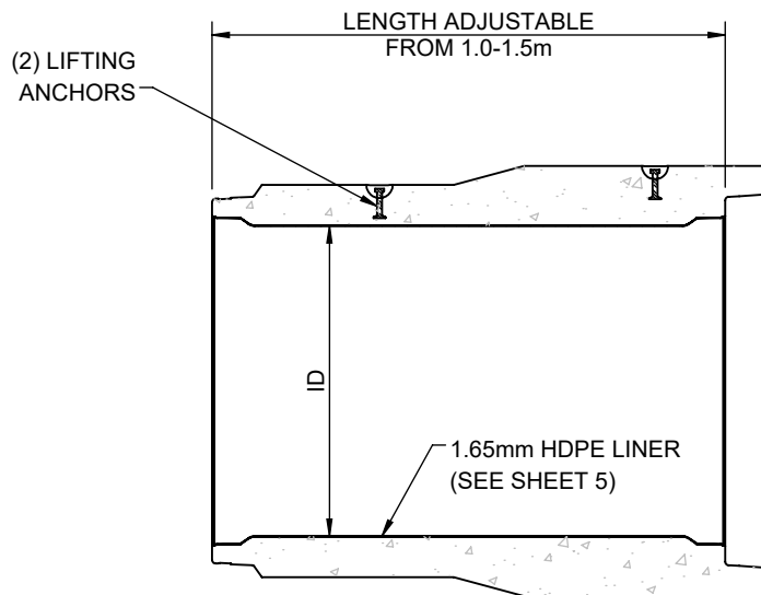
SECTION VIEW
