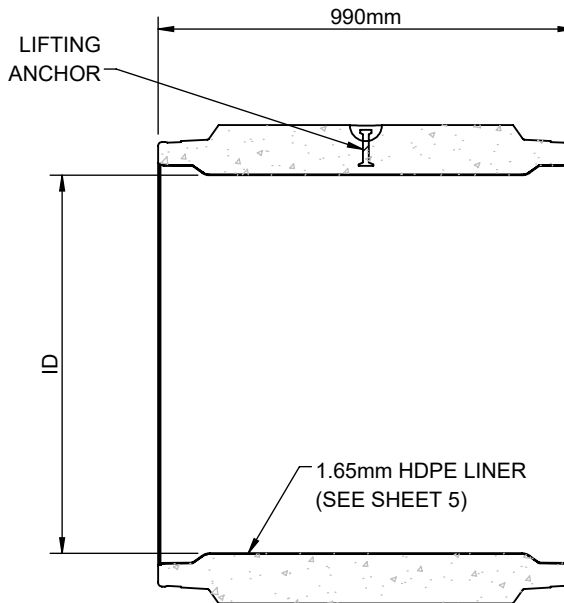
SECTION VIEW
