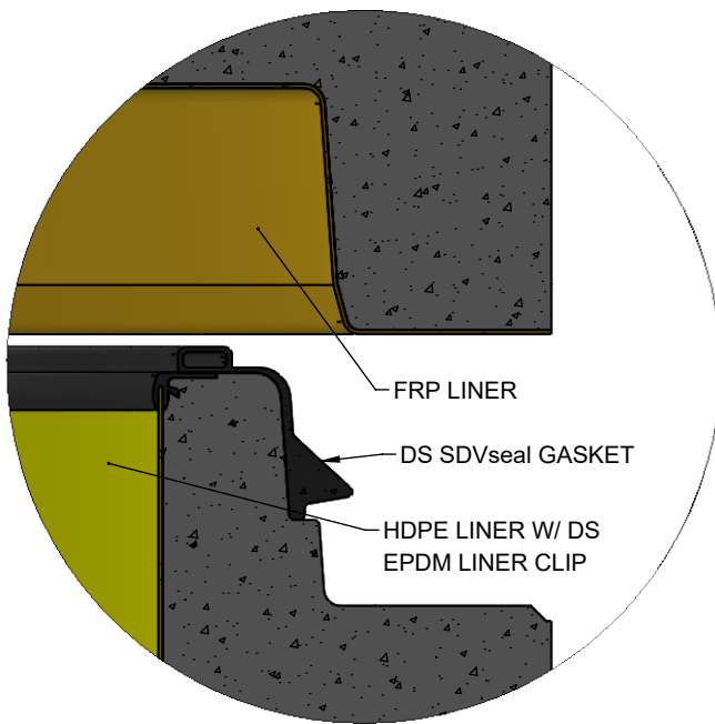
RISER TO FLAT LID JOINT DETAIL
