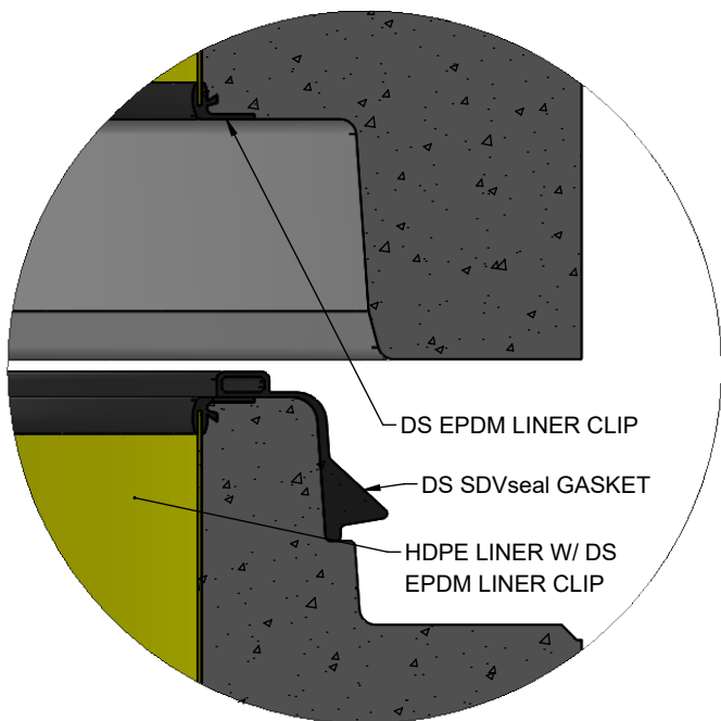
RISER TO RISER JOINT DETAIL
