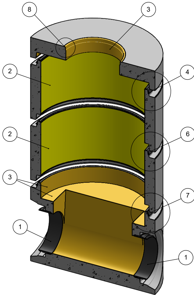
MANHOLE WITH FLAT LID
