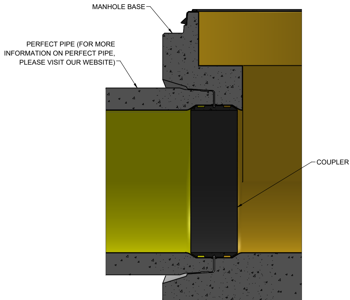
INTERNAL COUPLER PERFECT PIPE CONNECTOR
