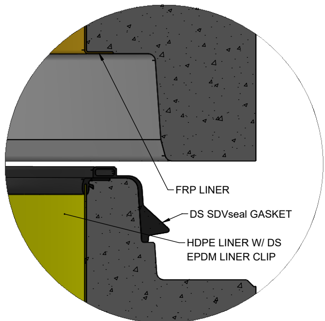
RISER TO CONE JOINT DETAIL
