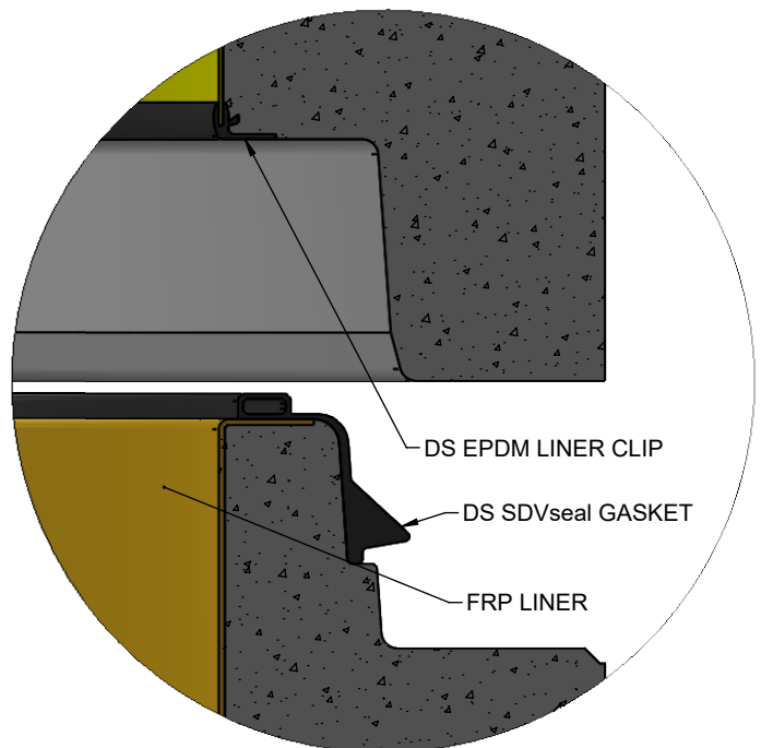
BASE TO RISER JOINT DETAIL
