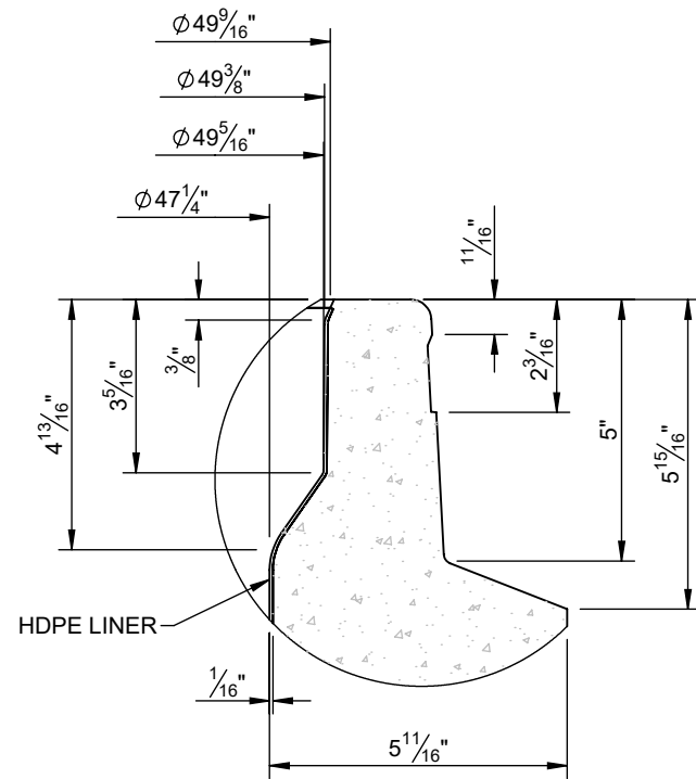
SPIGOT DETAIL (SCALE 1 : 4)
