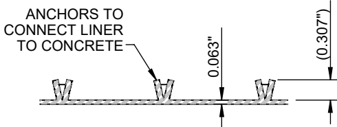
HDPE LINER DETAIL WITH ANCHORS
