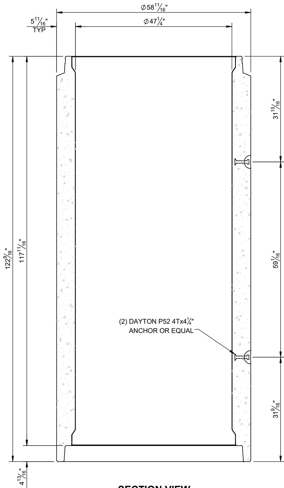
SECTION VIEW
