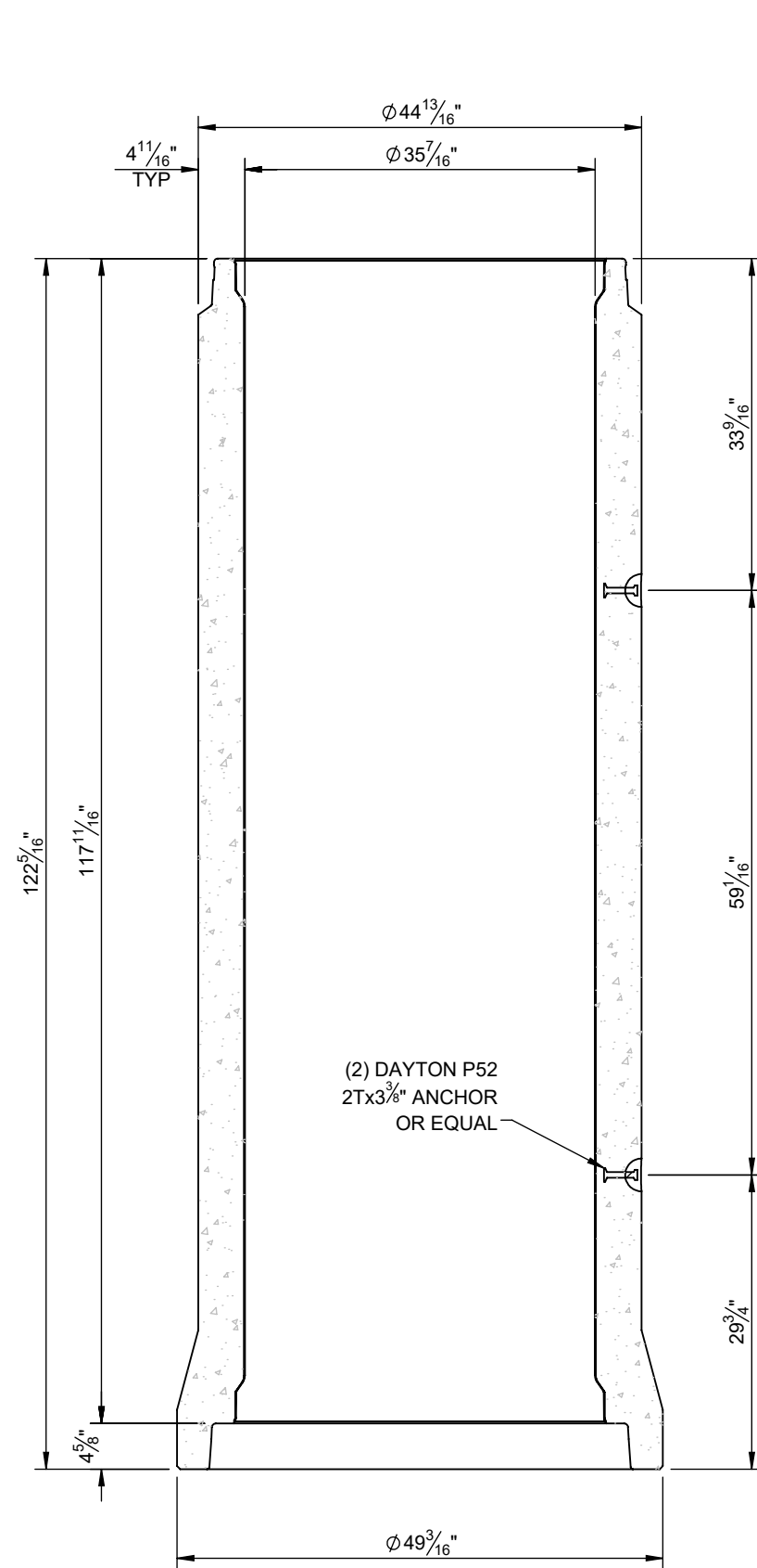
SECTION VIEW
