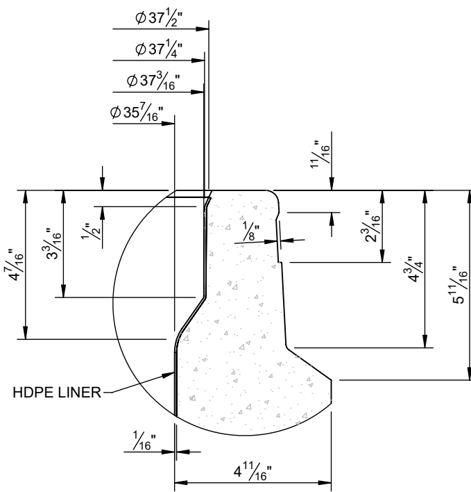
SPIGOT DETAIL (SCALE 1 : 4)
