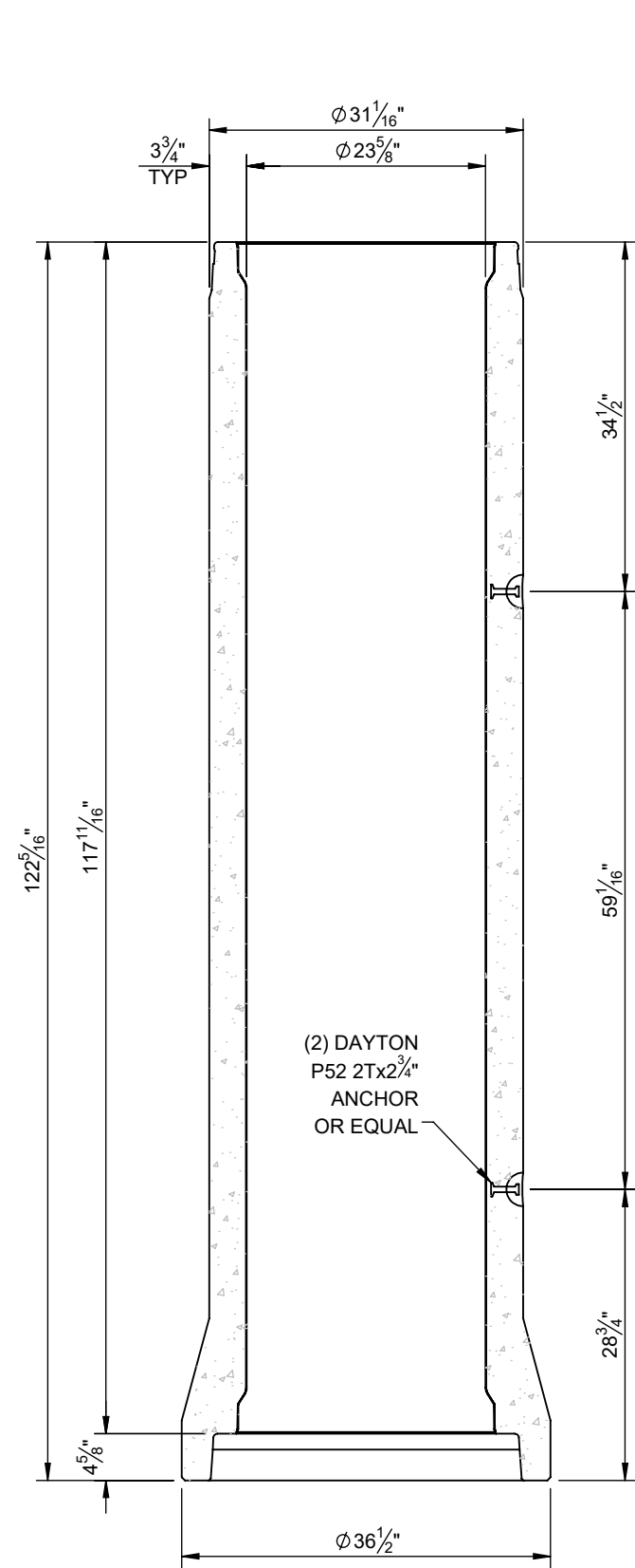
SECTION VIEW
