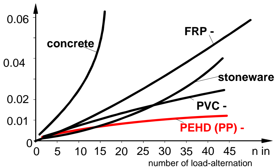
diagram1: Comparison of the abrasion of Polyethylene (PEHD) & Polypropylene (PP) with other materials, tested acc. to "Darmstädter" test method
