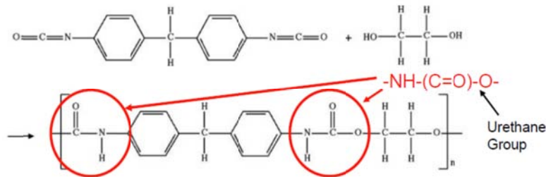
Figure 1: Linking Molecular Units by Urethane Groups (Rahman, 2011)
