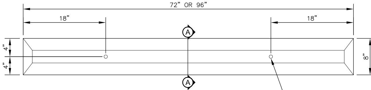
PLAN VIEW
