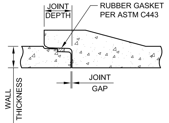
SECTION B-B NRCP JOINT DETAIL
