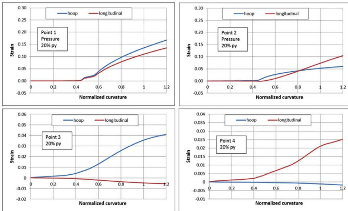
Figure 14. Evolution of local strain at critical locations of welded lap joints subjected to severe bending ( D/t = 191 ; “double weld”; internal pressure equal to 20% of yield pressure).
