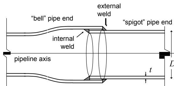
Figure 1. Configuration of a double-welded lap pipe joint.
