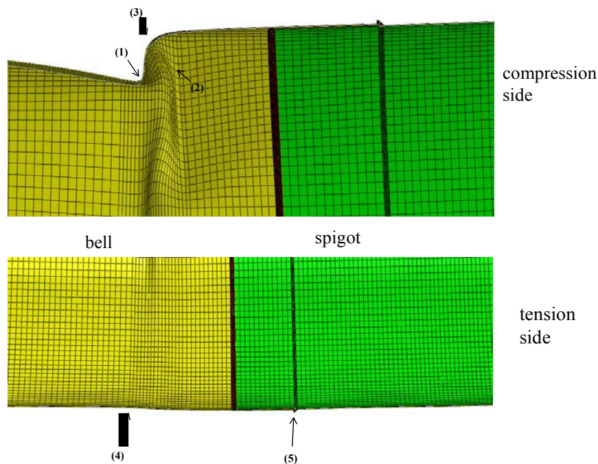
Figure 11. Critical locations in welded lap joints subjected to bending under zero pressure ( D/t = 191 ).
