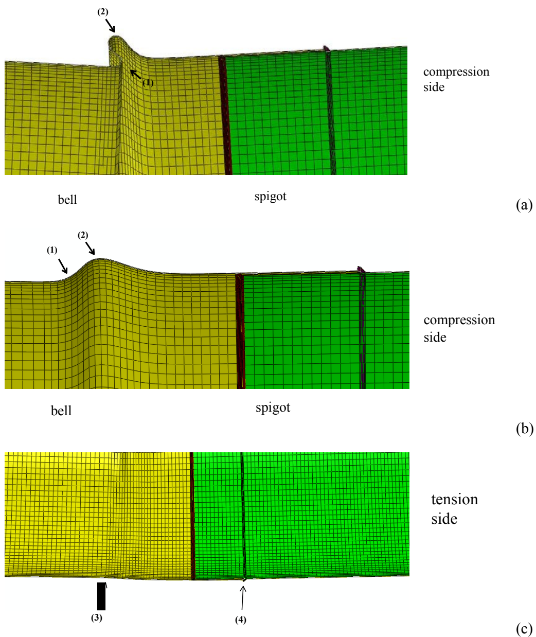
Figure 12. Critical locations in welded lap joints subjected to bending; (a) and (c) refer to pressure equal to 20% of yield pressure; (b) and (c) refer to pressure equal to 40% of yield pressure
