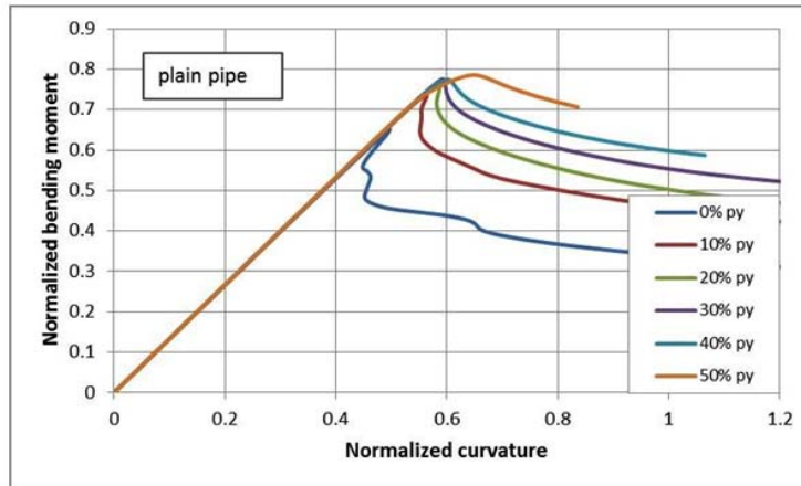
Figure 4. Bending response in the presence of internal pressure of pipe; initial wrinkling amplitude equal to 30% of pipe thickness ( D/t = 191 ).
