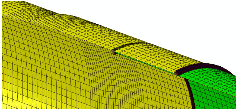
Figure 2. Finite element model for welded lap joint simulation; geometry of the double weld area.
