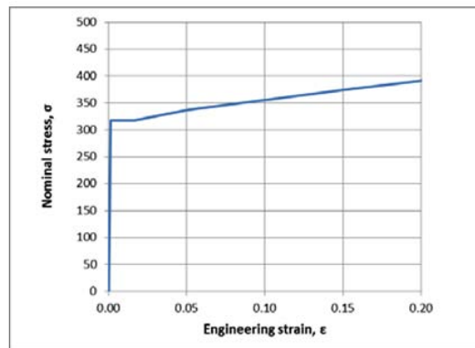
Figure 3. Stress- strain curve of ASTM 1018 grade 46 steel used in the present analysis; yield stress is equal to 317 MPa [46,000 psi].
