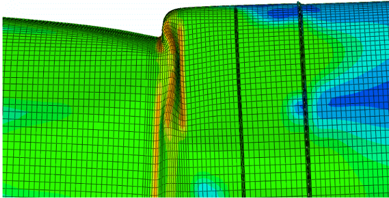
Figure 8. Deformed shape of a welded lap joint subjected to bending loading, characterized by localization of deformation; D/t = 191 , zero pressure.
