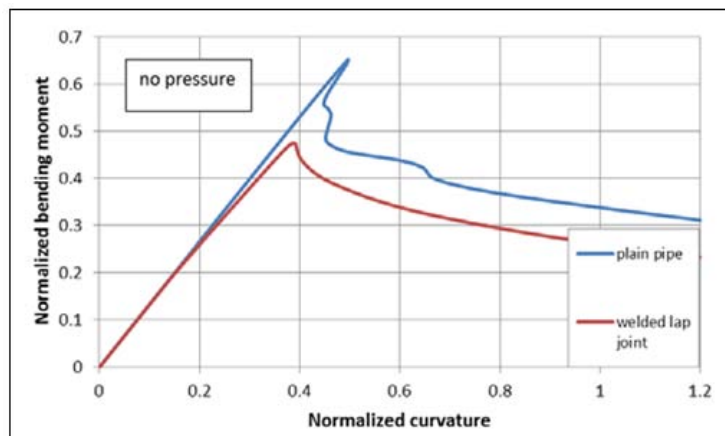
Figure 7. Moment-curvature diagrams for plain pipe and double-welded joints ( D/t = 191 , zero pressure).
