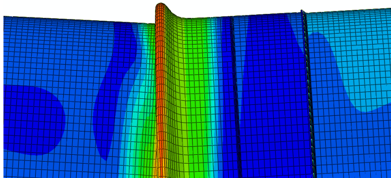
Figure 10. Effect of pressure on deformed shape of welded lap joint subjected to bending loading; compression side of the pipe ( D/t = 191 ).
