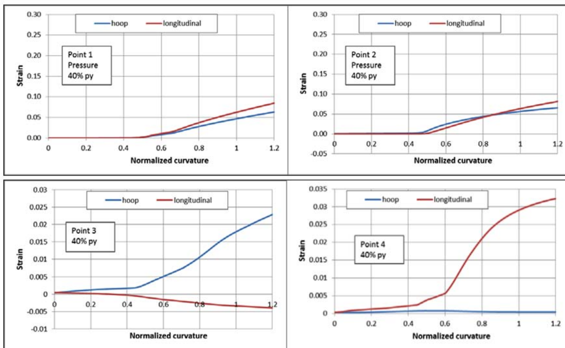
Figure 15. Evolution of local strain at critical locations of welded lap joints subjected to severe bending ( D/t = 191 ; “double weld”; internal pressure equal to 40% of yield pressure).
