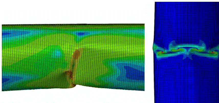
Figure 5. Plain pipe with D/t equal to 191 and initial wrinkling equal to 30% of pipe thickness.
