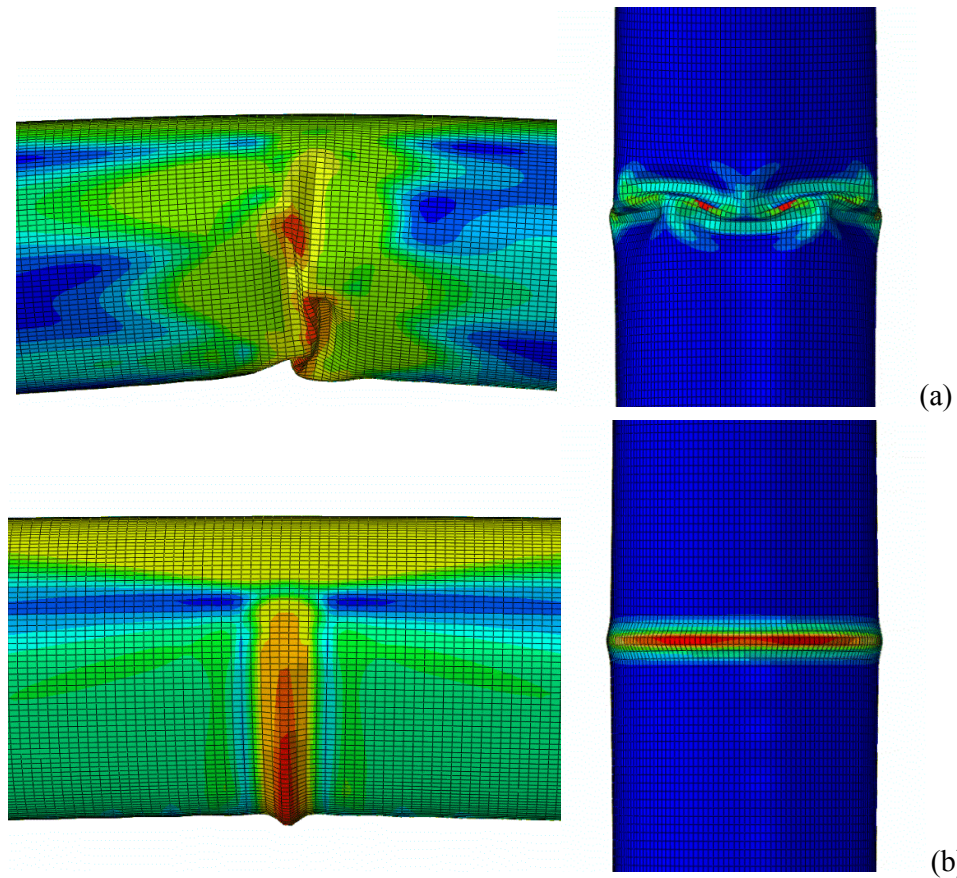
Figure 6. Buckling shape of a plain pipe in the presence of pressure (a) 10% of yield pressure, (b) 50% of yield pressure ( D/t = 191 ).
