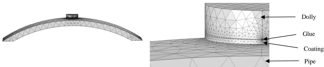
Figure 2. Overall and detailed view of the mesh used in the finite element computer simulation of the pull-off test on a pipe. The coating beyond the scoring around the dolly is not included since it is separated from the coating under stress.
