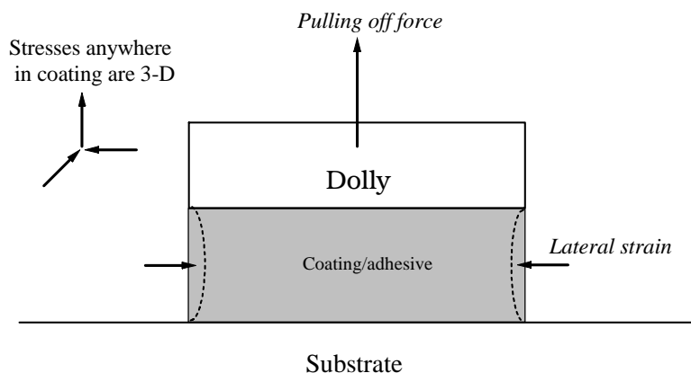
Figure 1. Schematic of the pull-off adhesion test illustrating how constraints produced by adhering to a rigid substrate and a rigid dolly cause multi-directional strains in the deformable coating and glue.
