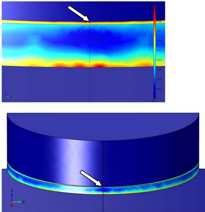
Figure 4. When the coating and glue have the same modulus, the maximum value of the first principal strain is at the glue-dolly intersection, over the crest in the pipe. Includes expanded view.
