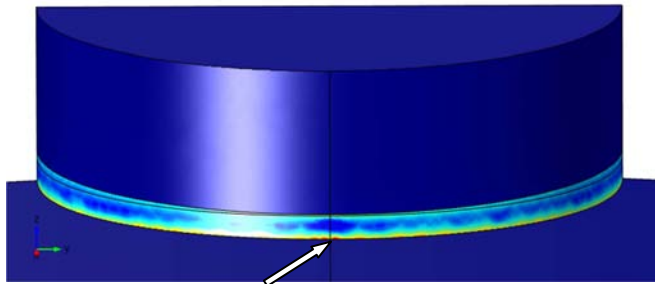
Figure 3. Distribution of the first principal strain in the coating between a level dolly and the steel pipe. The arrow indicates the position of the maximum tensile strain.
