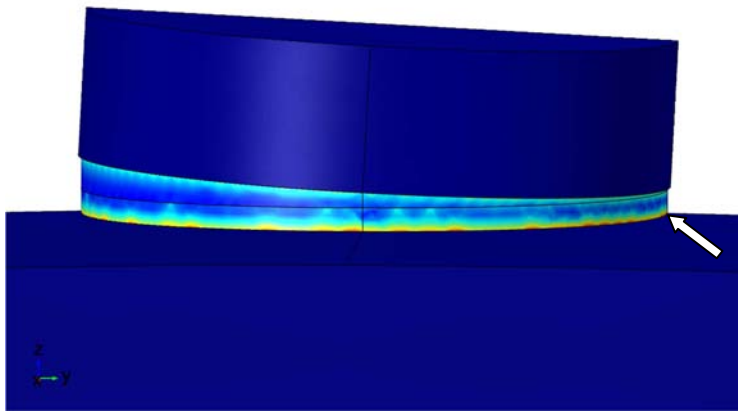
Figure 5. Distribution of first principal strain under a dolly adhering with a slanted glue line. The maximum value of the first principal strain is where the glue line is the thinnest.
